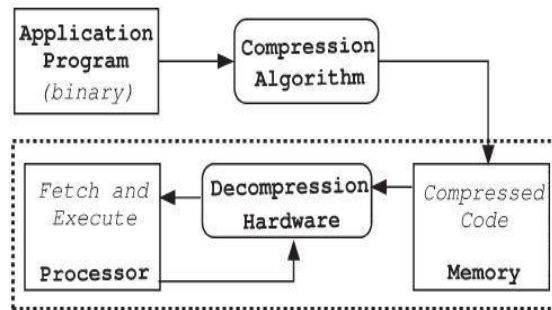
Fig. 1. Code-compression methodology.
