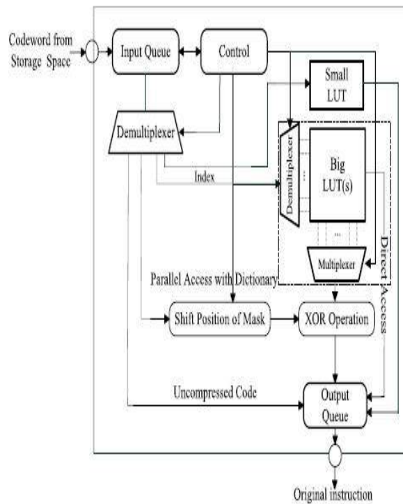
Fig 7 Logic diagram of decompression engine.
