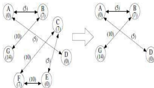
Fig 4 Bit-Saving Dictionary Selection Method
